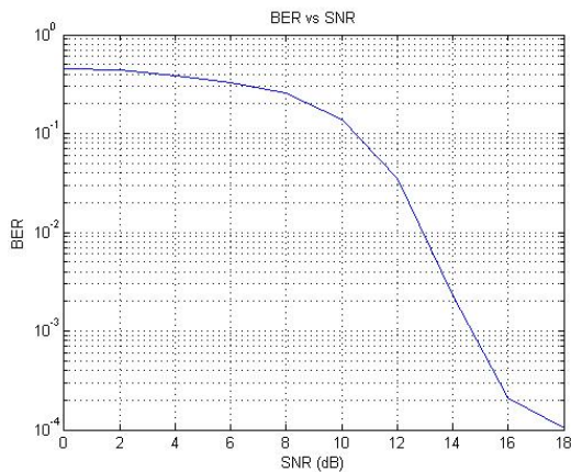
Figure 2.1: Simulation results of SNR with BER
