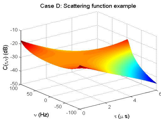
Figure 2.4: Channel Estimation using Scattering Function
