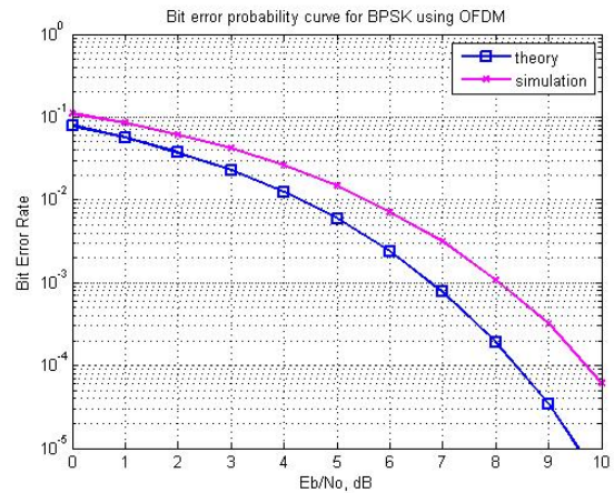
Figure 2.2: Simulation results BER with AN Product.
