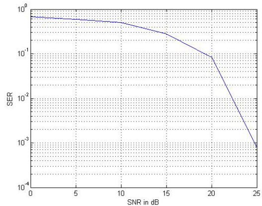
Figure 2.6: Simulated BER with 1/2-rate convolution coding
